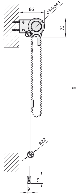
Detail Wandmontage
